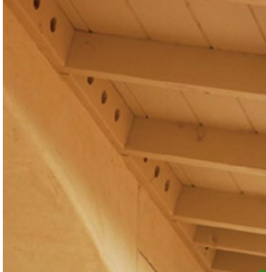
UNENCLOSED EAVES
